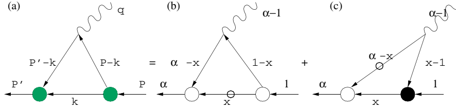
FIG. 1 (color online). Covariant triangle diagram (a) is represented as the sum of LF valence diagram (b) defined in the 0 < k^+ < P^+ region and the nonvalence diagram (c) defined in the P^+ < k^+ < P'^+ region, where \alpha = P'^+/P^+ = 1 + q^+/P^+ . The large white and black blobs at the meson-quark vertices in (b) and (c) represent the ordinary LF wave function and the nonvalence wave function vertices, respectively. The small white blobs in (b) and (c) represent the (on-shell) mass pole of the quark propagator determined from the k^- integration.
