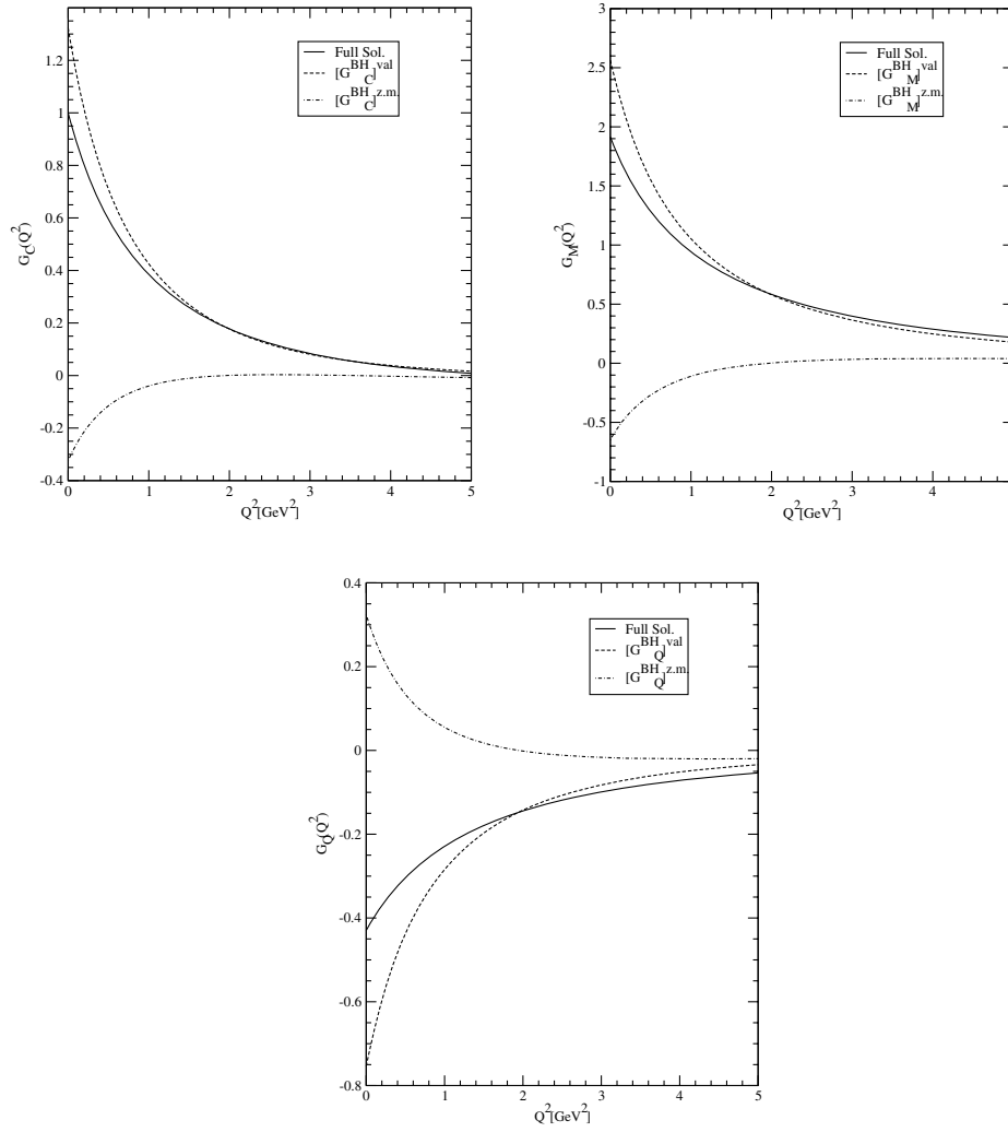
FIG. 3. Form factors of the \rho meson, i.e., charge [G_C(Q^2)] , magnetic [G_M(Q^2)] , and quadrupole [G_Q(Q^2)] form factors. The solid and dashed lines represent the full (i.e., valence + zero mode) solution and valence contribution ( I_{00}^{+val} ) to the form factors, respectively. The dash-dotted line represents the zero-mode contribution, i.e., full solution – valence contribution.
