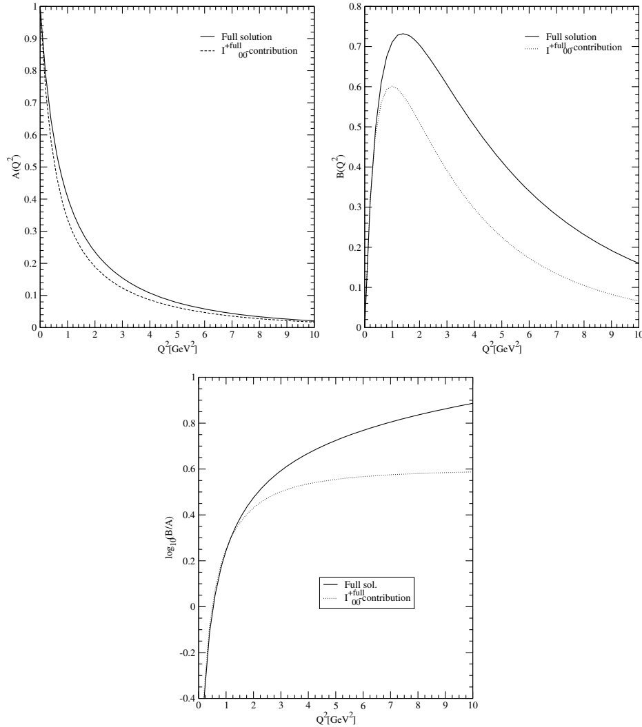
FIG. 4. Structure functions A(Q^2) , B(Q^2) , and their ratio \log_{10}(B/A) . Solid and dotted lines represent the full results and the contributions only from the I_{00}^{+\text{full}} = I^{+\text{val}} + I^{+\text{z.m.}} component.
