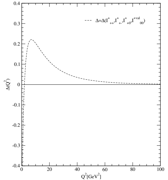
FIG. 2. The angular condition given by Eqs. (4) or (29) in the Breit frame, i.e., \Delta(Q^2) = I_{00}^{+\text{z.m.}} . Note that the zero-mode contribution is necessary to satisfy the angular condition even at Q^2 = 0 , where \Delta(0) = -0.65 in our model calculation.
