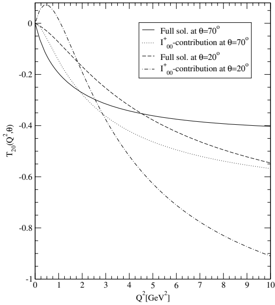
FIG. 5. Tensor polarization T_{20}(Q^2) at \theta = 70^\circ (solid line) and \theta = 20^\circ (dashed line). For comparison, we also show the I_{00}^+ dominance at \theta = 70^\circ (dotted line) and \theta = 20^\circ (dot-dashed line).
